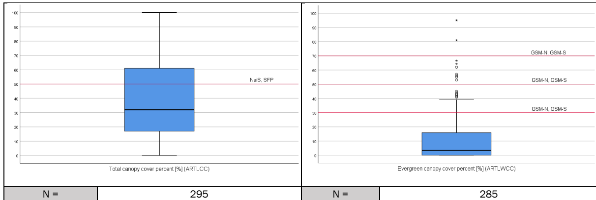
Figure 322-4: Observed forest avalanches – canopy cover percent on release areas
