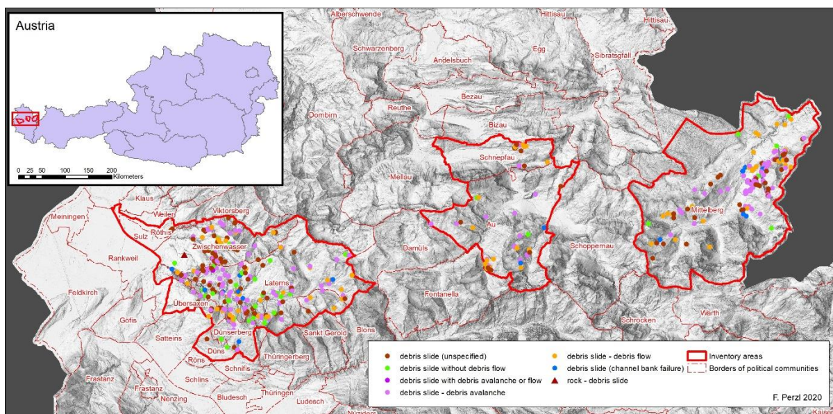
Figure 22-1: Forest landslide examples
