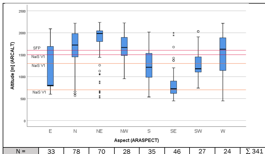
Figure 321-2: Boxplots of elevations of forest avalanche initiations
